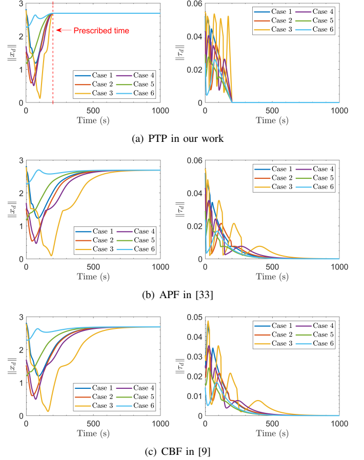
Fig. 7. Control responses of different path planners.
